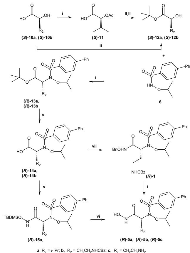
Scheme 2. Reagents and conditions: (i) \text{AcCl} , rt, 18 h; (ii) (\text{CH}_3)_2\text{NCH}[\text{O}(\text{CH}_3)_3]_2 , toluene, 95^\circ\text{C} , 3 h; (iii) \text{LiOH} , \text{THF}/\text{MeOH}/\text{H}_2\text{O} , rt, 3 h; (iv) \text{TPP} , \text{DEAD} , anhyd \text{THF} , 0^\circ\text{C} , 5 h; (v) \text{TFA} , anhyd \text{DCM} , 0^\circ\text{C} , 5 h; (vi) \text{TBDMSiONH}_2 , \text{EDCI} , anhyd \text{DCM} , 0\text{--}25^\circ\text{C} , 24 h; (vii) \text{TFA} , anhyd \text{DCM} , 0^\circ\text{C} , 5 h; (viii) \text{BnONH}_2\text{HCl} , \text{NMM} , \text{HOBT} , \text{EDCI} , anhyd \text{DCM} , rt, 24 h; (ix) \text{H}_2 , \text{Pd/C} 10%, \text{MeOH}/\text{AcOH} .
